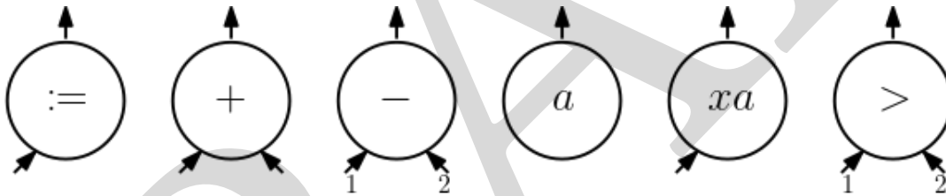
Figure 22.4: The operation vertices of ARITH CIRCUIT SAT.
