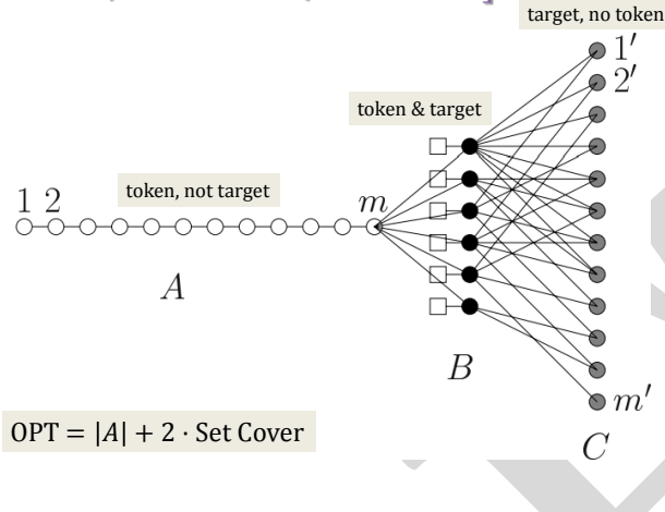
Figure 9.7: L -Reduction from SET COVER to MOTION PLANNING modified.
