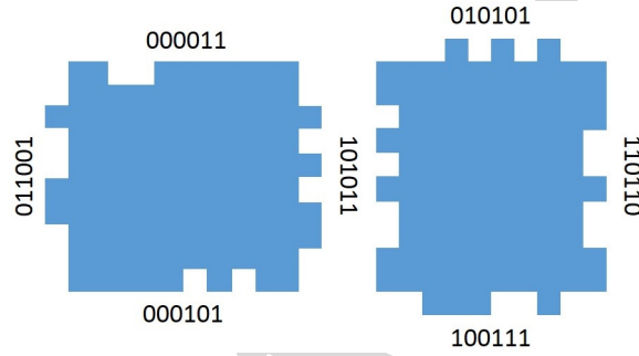
Figure 5.13: Encoding of jigsaw pieces into polyominoes.
