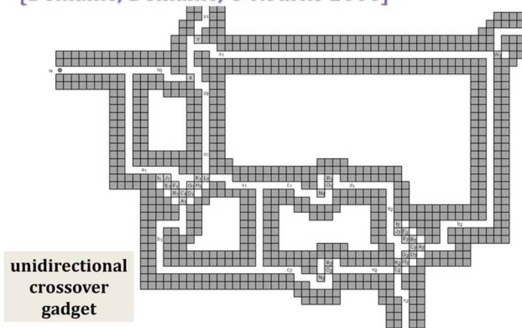
Figure 1.8: Unidirectional crossover gadget.
