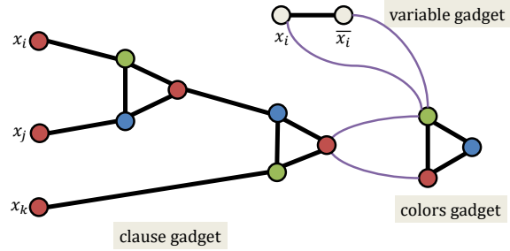
(b) Unsatisfying assignment for clause x_i \vee x_j \vee x_k
