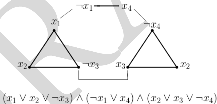
Figure 9.1: L-Reduction from MAX 3SAT-3 to INDEPENDENT SET-B-4.
