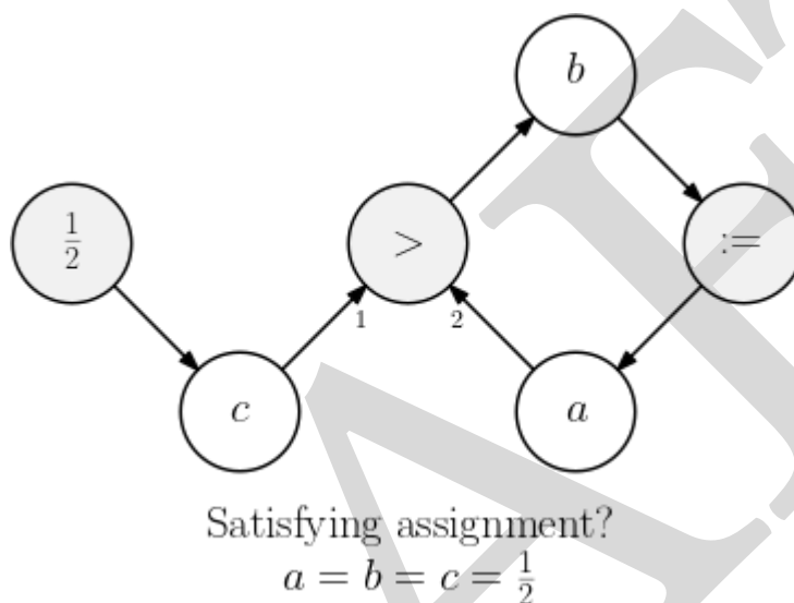
Figure 22.5: The operation vertices of ARITH CIRCUIT SAT.
