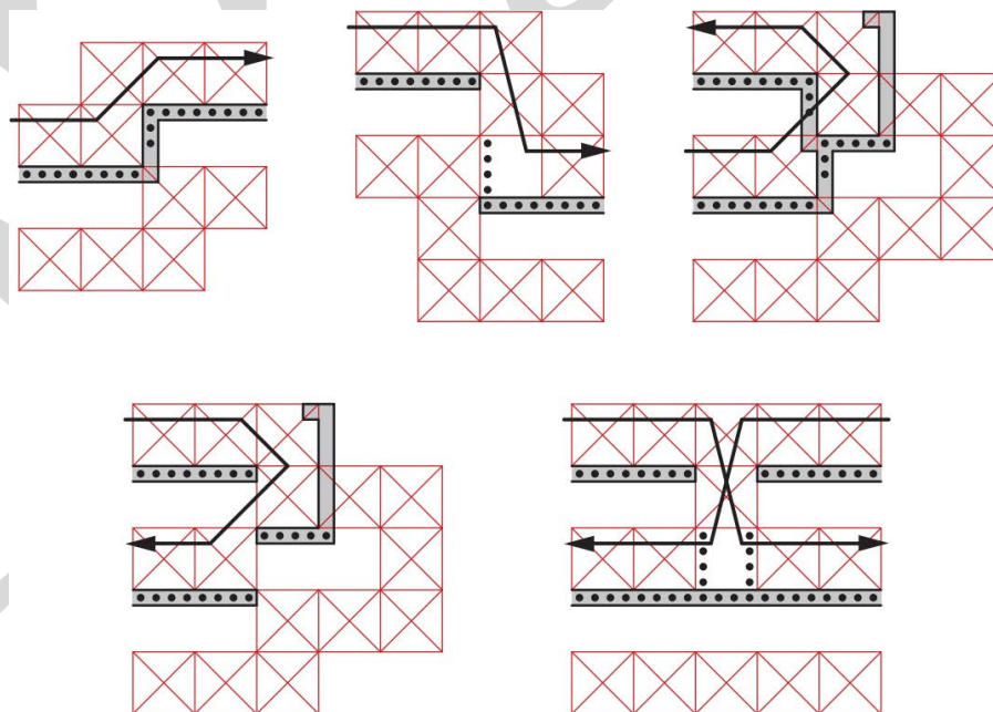
Figure 13.8: Upper: Builder Gadget; Lower: Path Gadget
