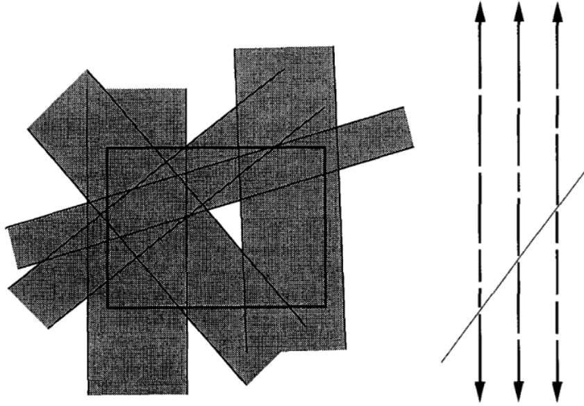
Figure 17.6: Reduction from GEOMBASE' to STRIPS.
