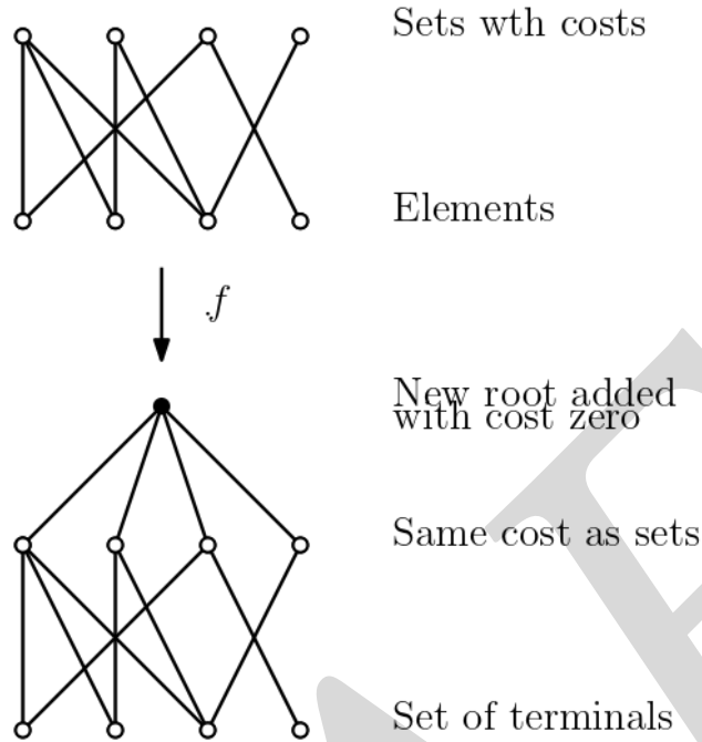
Figure 9.8: APX-Reduction from SET COVER to NWST.
