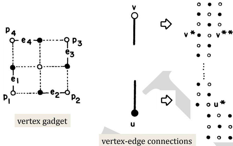
Figure 4.6: Vertex gadget.
