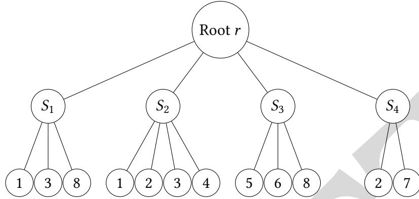
Figure 9.9: L -Reduction from SET COVER to GST.
