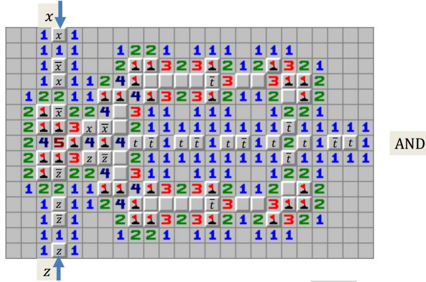
Figure 3.7: Minesweeper AND gate.
