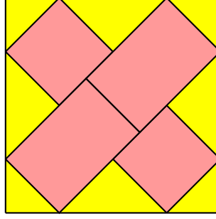
Figure 5.4: An example of rectangle packing.
