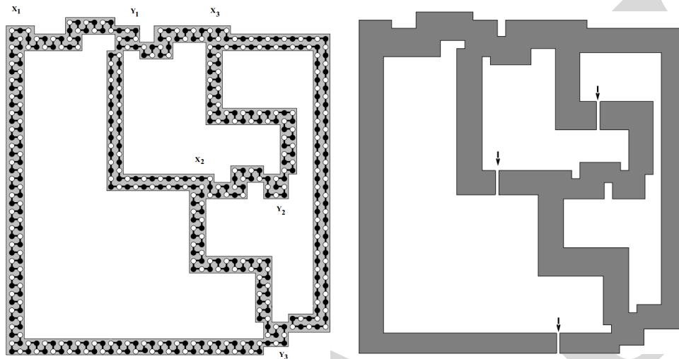
Figure 4.14: Milling and lawn mowing are NP-complete.
