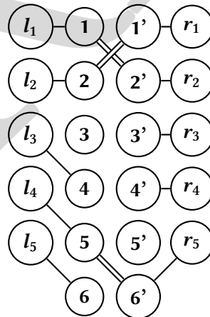
Figure 20.3: Instance of PERF_MAT( G ) based on INDEX( x , 3, 5).
