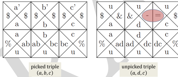
Figure 9.5: Gadgets for EM \leq_L 3D \text{ MATCHING} .
