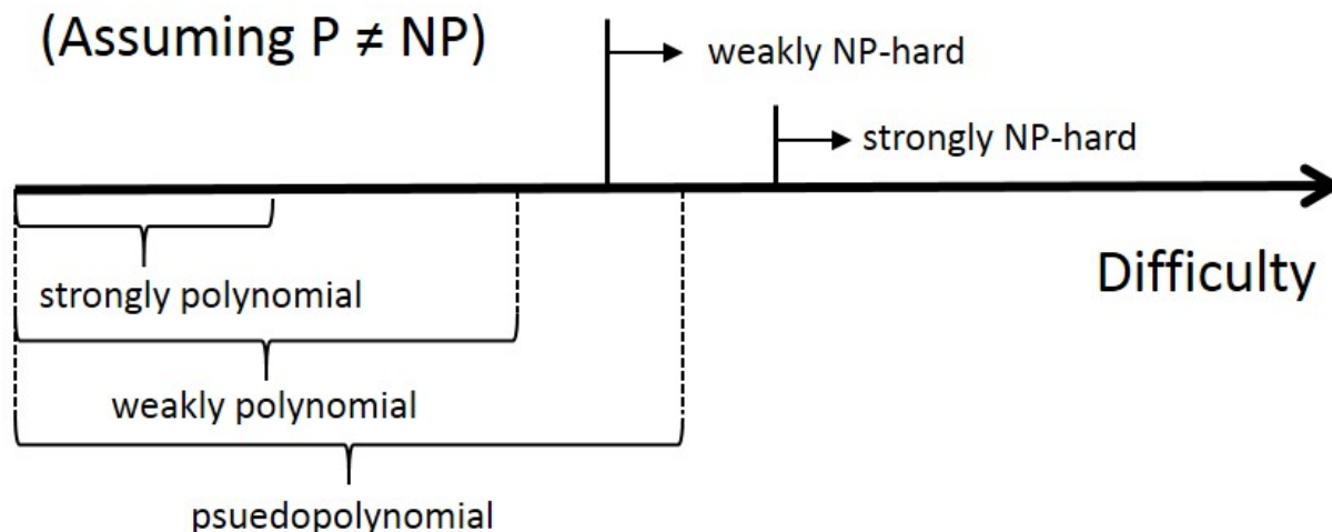
Figure 5.1: Relationships between types of polynomial time and NP-hardness.
