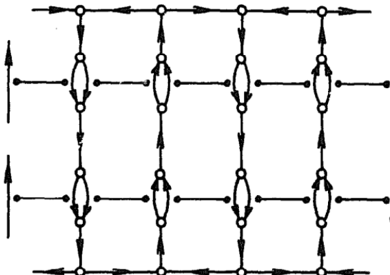
Figure 4.1: Gadgets for proving HAMILTONIAN CYCLE on planar maximum-degree-3 graphs is NP-complete.
