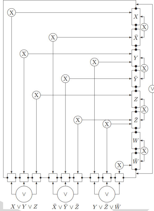
Figure 11.3: Example.
