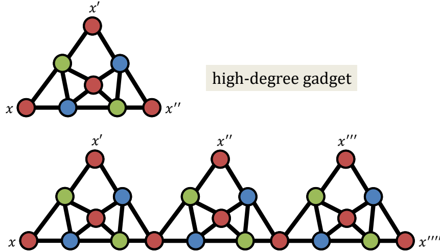
Figure 2.4: Gadget for reducing maximum degree to 4.
