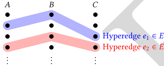
Figure 2.16: 3D MATCHING.
