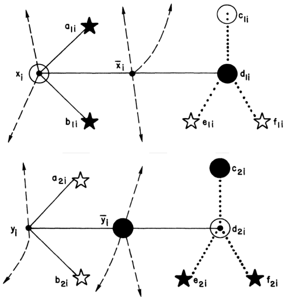
Figure 14.2: Variable gadgets
