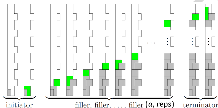
Figure 5.18: Gadget representing a_i in Tetris.
