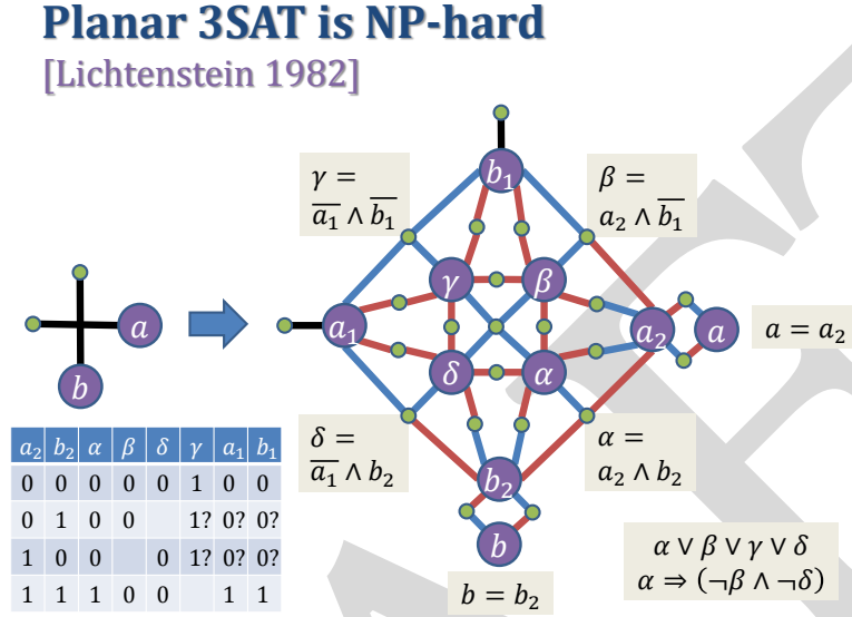
Figure 2.6: PLANAR 3SAT crossover gadget.
