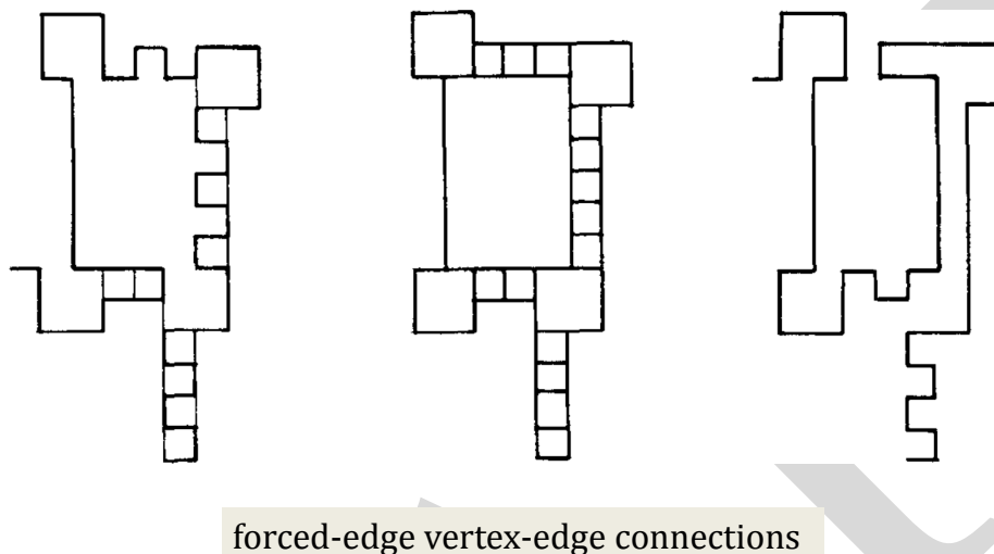
Figure 4.10: Forcing gadget for maximum-degree-3 grid graphs.
