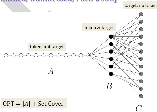
Figure 9.6: L -Reduction from SET COVER to MOTION PLANNING.
