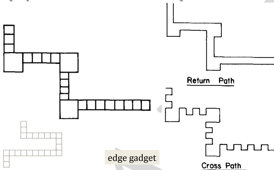
Figure 4.8: Edge gadget for maximum-degree-3 grid graphs.
