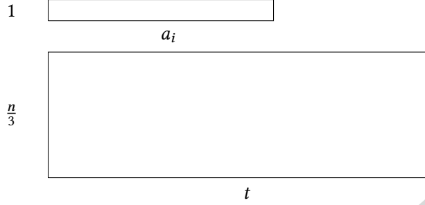
Figure 5.5: Reduction from 3-PARTITION to RECTANGLE-RECTANGLE PACKING without rotation.
