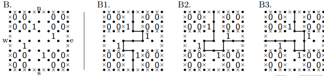
Figure 4.13: Slitherlink is NP-complete.
