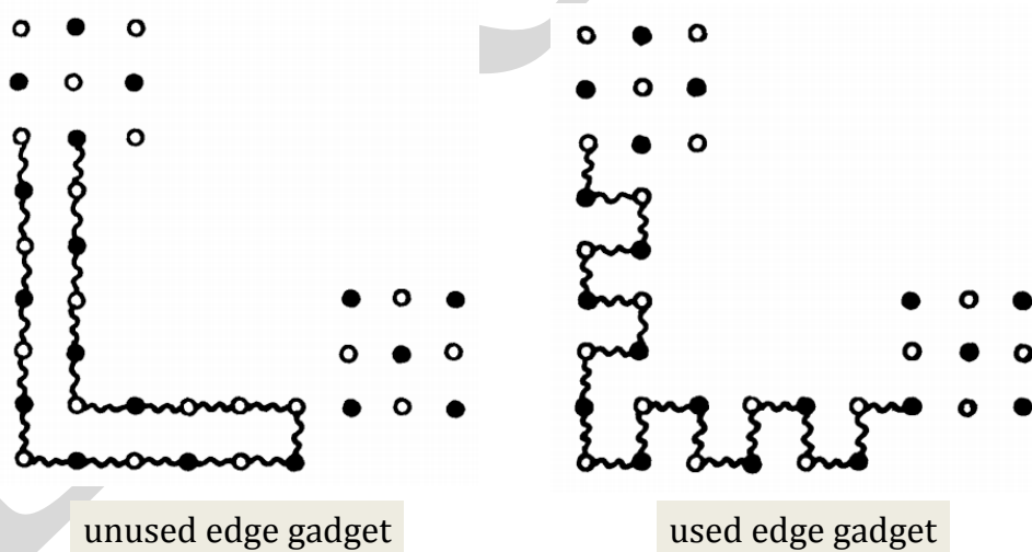
Figure 4.7: Hamiltonian grid graph.
