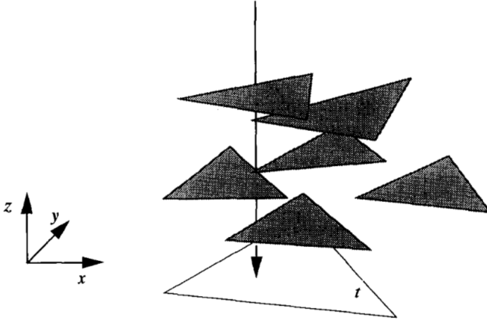
Figure 17.8: Reduction from VisTRI to TriCovTRI.
