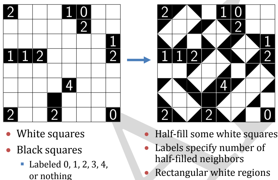
Figure 2.12: Example of Shakashaka puzzle.
