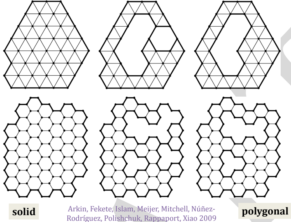
Figure 4.11: Polyagonal tiling.
