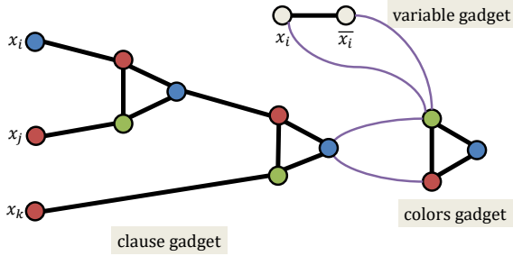
(a) Satisfying assignment for clause x_i \vee x_j \vee x_k
