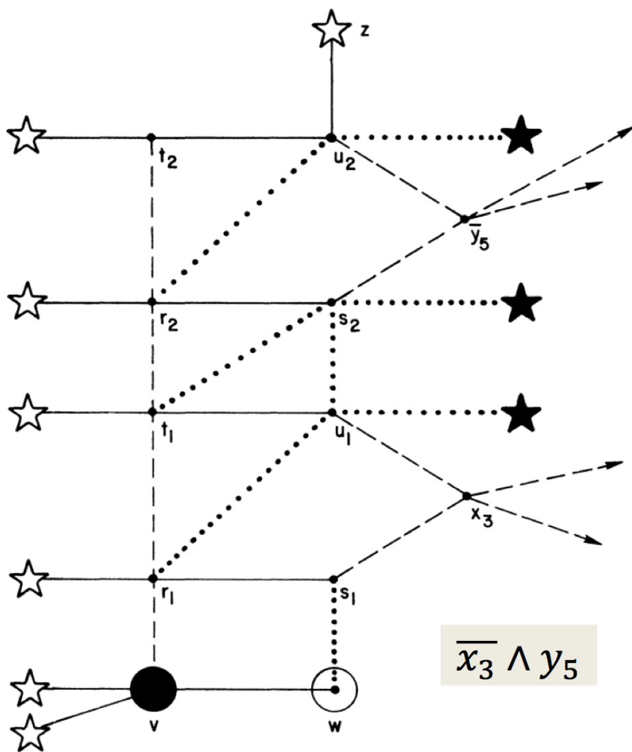
Figure 14.3: Gadget for the formula \overline{x_3} \wedge y_5
