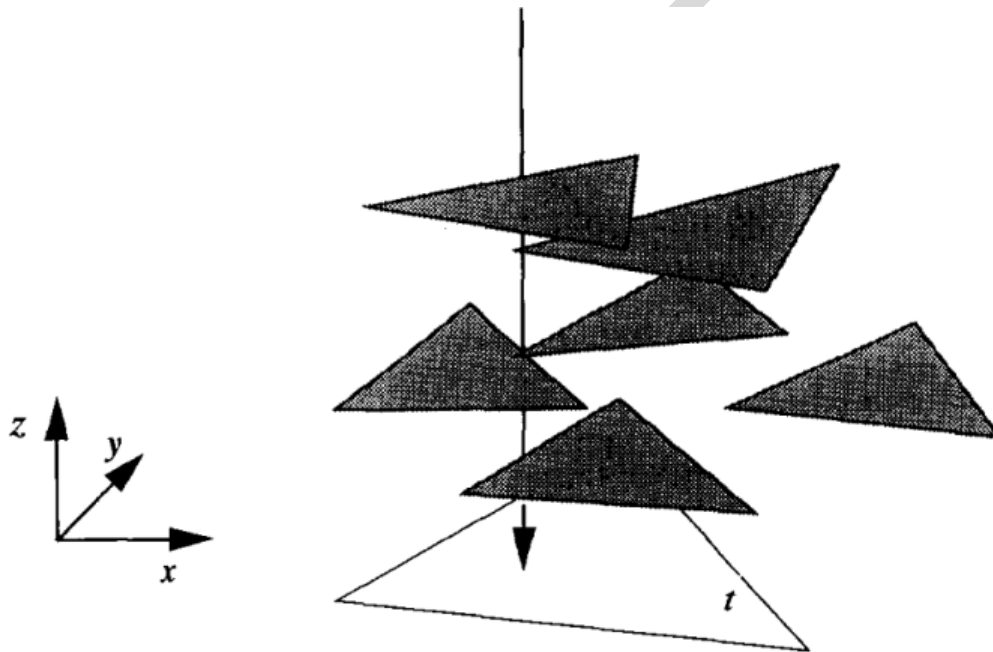
Figure 17.8: Reduction of \text{VisTri} to \text{TriCovTri} .
