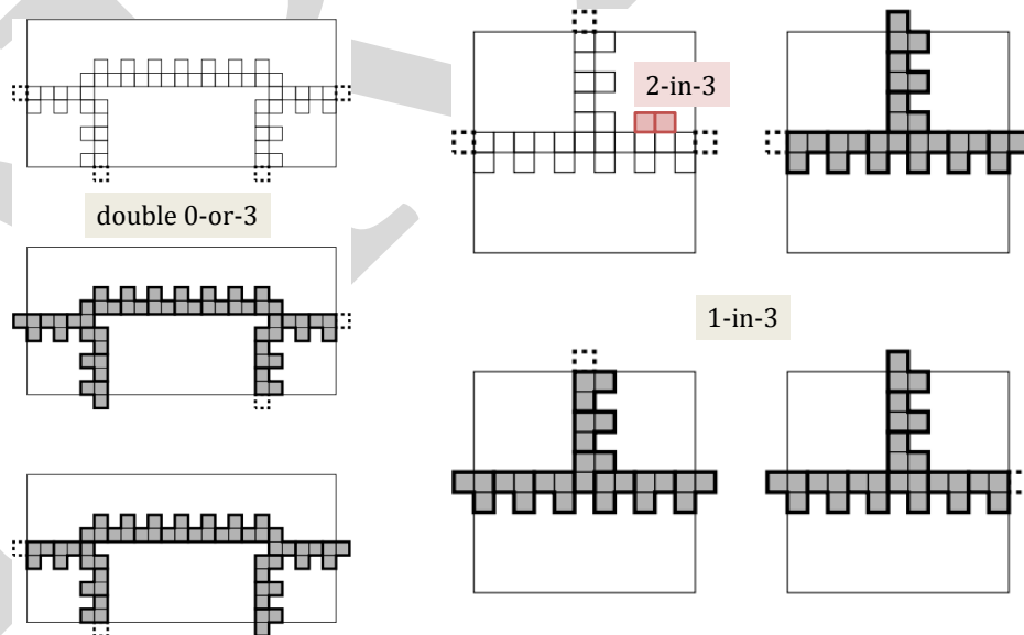
Figure 5.9: Gadgets for reduction of GRAPH ORIENTATION to L -TROMINOES PACKING.
