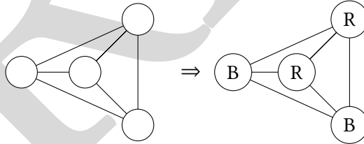
Figure 1.2: A graph that has a 2-colorable perfect matching.
