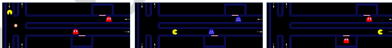
Figure 4.17: Token+Toll road gadget for Pac-Man.
