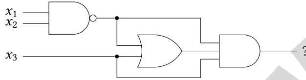
Figure 1.1: A boolean circuit.
