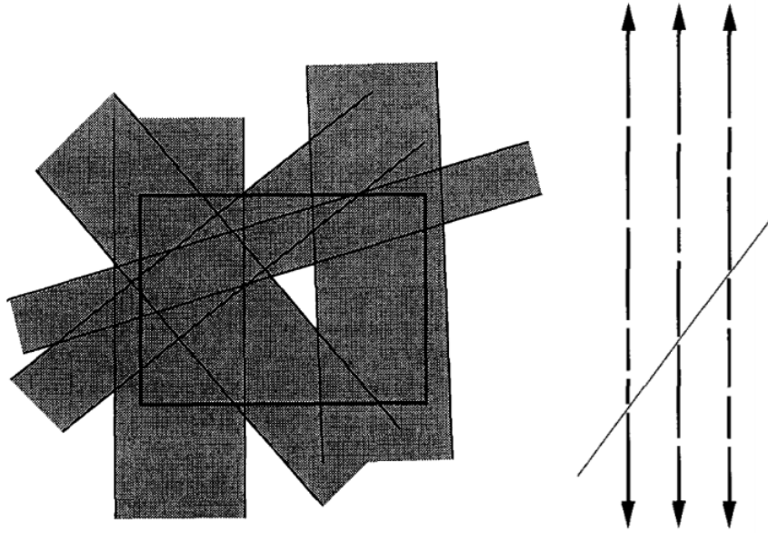
Figure 17.6: Reduction of GEOMBASE' to STRIPS.
