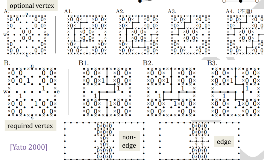
Figure 12.6: SLITHERLINK is #P-hard.
