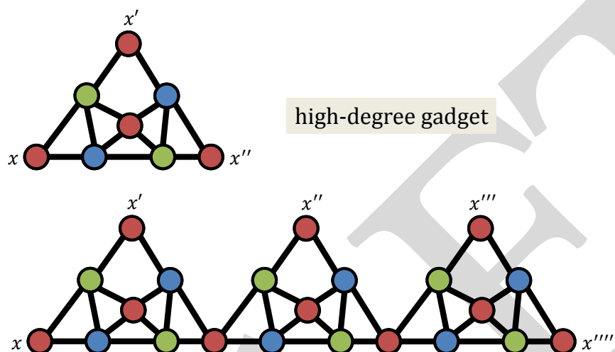
Figure 2.9: Gadget for reducing degree to 4.
