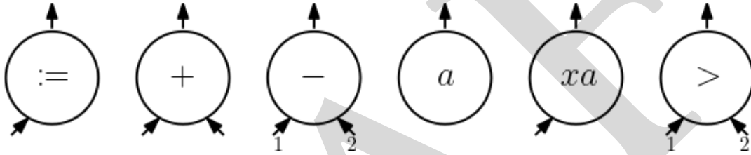
Figure 22.6: The operation nodes of ARITH CIRCUIT SAT.
