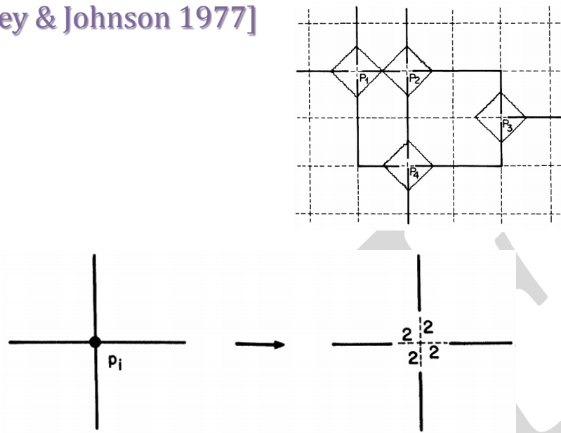
Figure 5.2: Transformation for RECTILINEAR EUCLIDEAN STEINER TREE.
