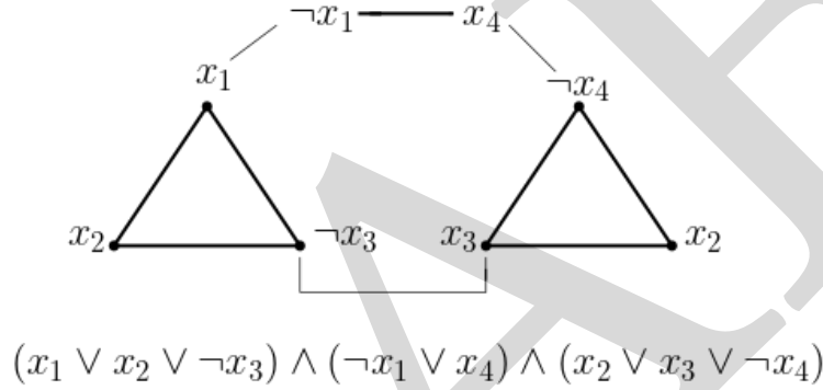
Figure 10.1: L -Reduction of MAX 3SAT-3 to INDEPENDENT SET-B-4.
