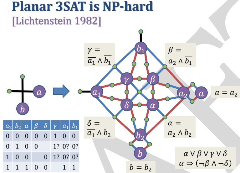
Figure 2.3: PLANAR 3SAT crossover gadget.
