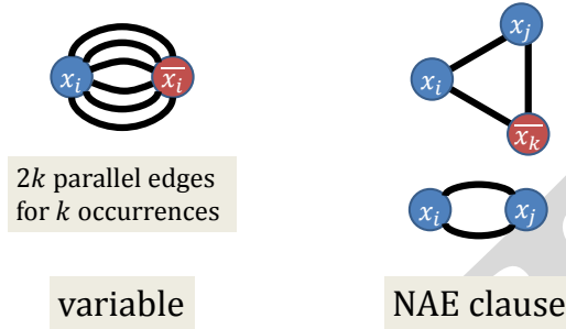
Figure 10.4: L -Reduction of MAX NAE-3SAT to MAXCUT.
