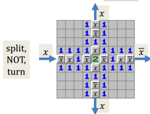
Figure 3.8: Split-Not-Turn gadget for Minesweeper.
