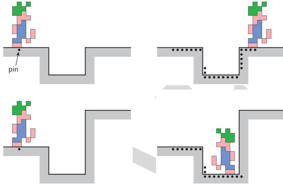
Figure 13.7: Lemmings Walker gadget for PSPACE-completeness.
