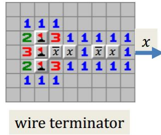
Figure 3.7: Termination gadget for Minesweeper.
