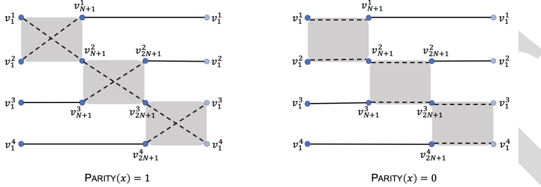
Figure 21.2: Reduction from a parity instance to a 1vsk-CYCLE instance with k = 4 .
