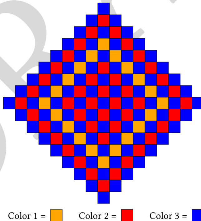
Figure 5.4: DIA(323132323).
