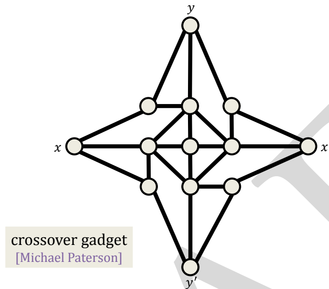
Figure 2.7: Crossover gadget.
