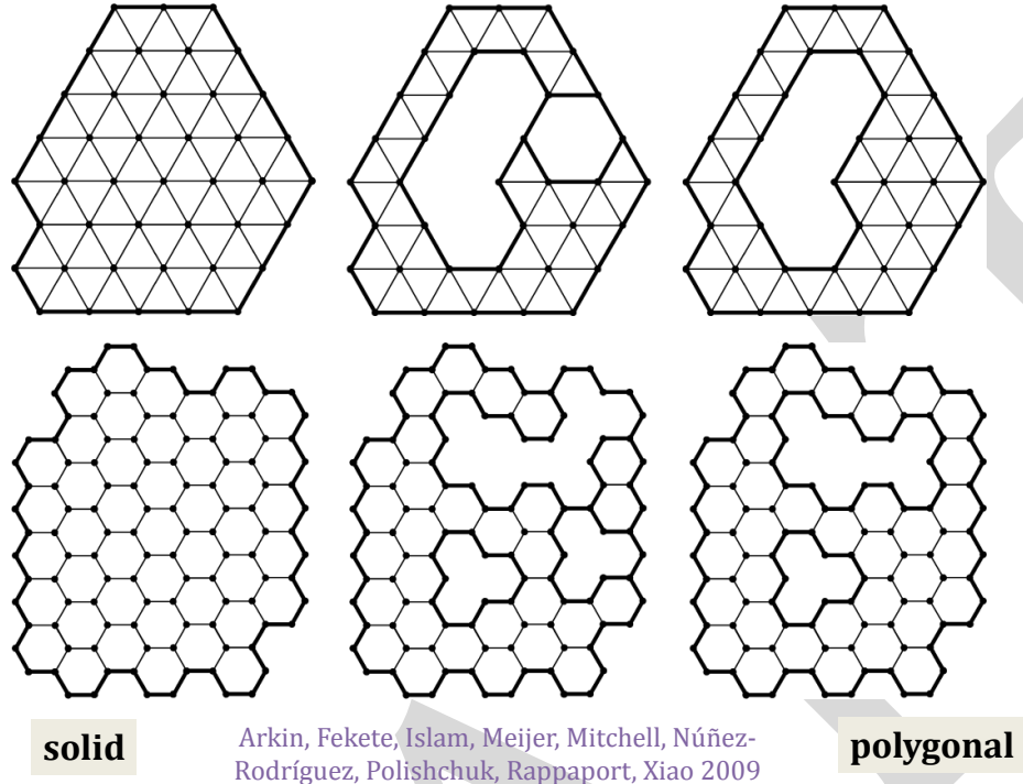
Figure 4.9: Polygonal tiling.
