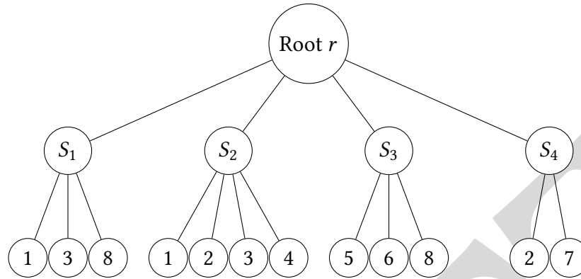
Figure 10.9: Reduction of SET COVER to GST.
