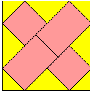
Figure 6.5: An example of rectangle packing.
