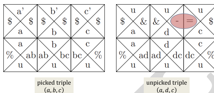
Figure 10.5: Gadgets for \text{EM} \leq_L \text{3D-MATCHING-2} .
