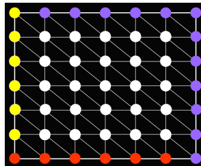
Figure 22.6: Valid Edge Coloring for the Sperner Edge Coloring
