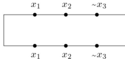
Figure 12.8: Gadgets For Variables in Proof PERM is #P-hard
