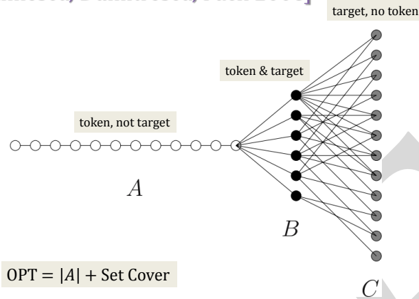
Figure 10.3: SET COVER \leq_L MOTION PLANNING
