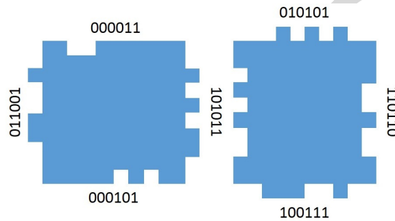
Figure 6.13: Encoding of Jigsaw Pieces into Polyominoes
