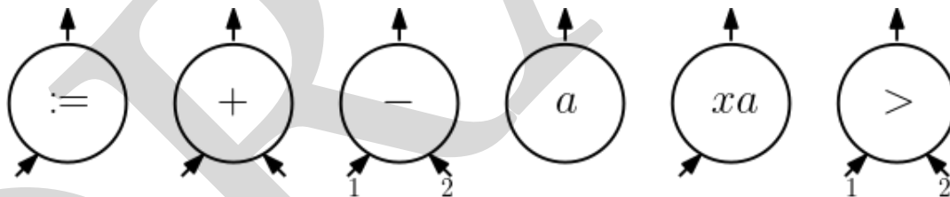
Figure 22.10: The Operation Nodes of ARITH CIRCUIT SAT
