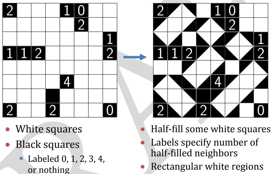
Figure 2.17: Example of Shakashaka Puzzle
