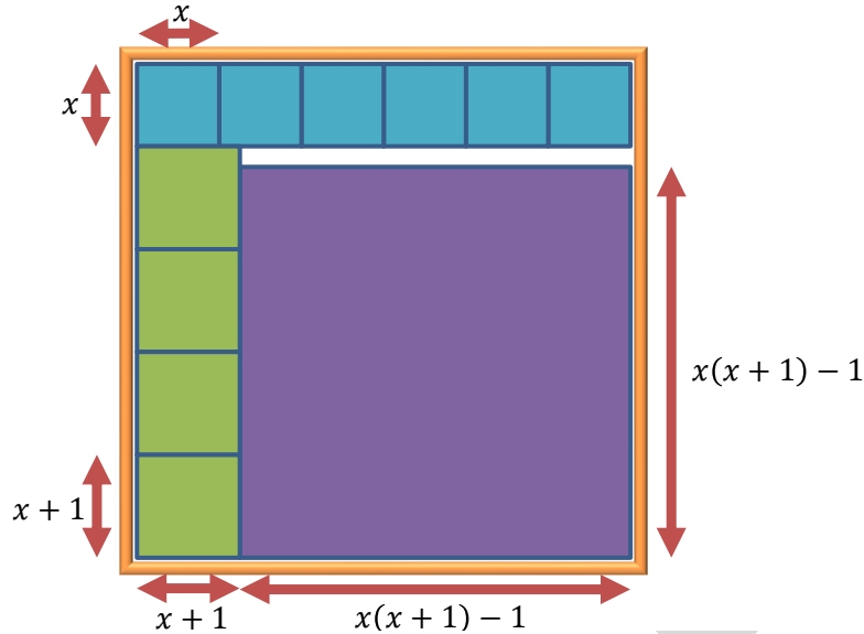
Figure 6.8: 3\text{-PARTITION} \leq \text{SQ-SQ PACKING}
