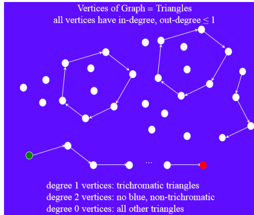
Figure 22.8: The Triangulation of Sperner's Lemma Turned into a Directed Graph
