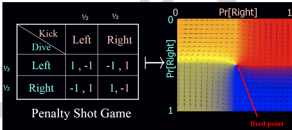
Figure 22.5: The Proof of Nash Using Brouwer
