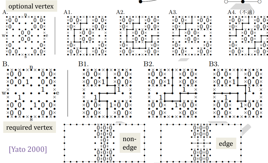
Figure 4.9: Slitherlink is NP-Complete
