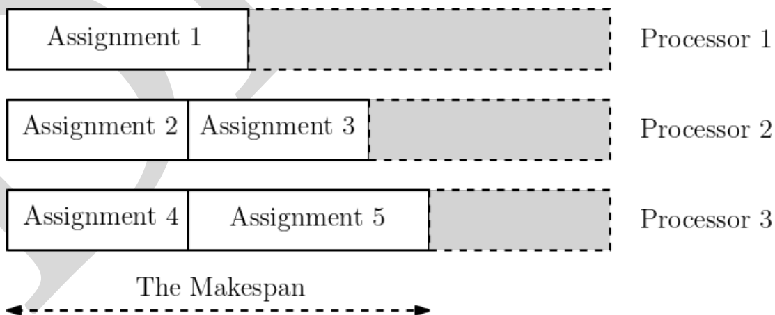
Figure 6.3: An Assignment of Processes to 3 Processors
