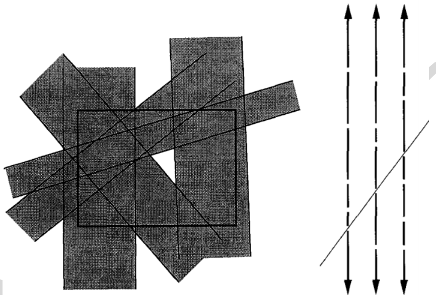
Figure 17.6: The Reduction from GEOMBASE to STRIPS Using GEOMBASE'
