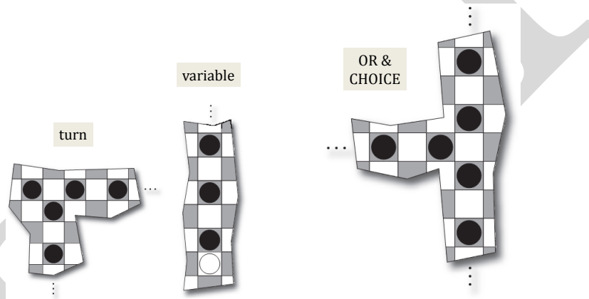
Figure 16.3: Gadgets to prove Konane PSPACE-Complete
