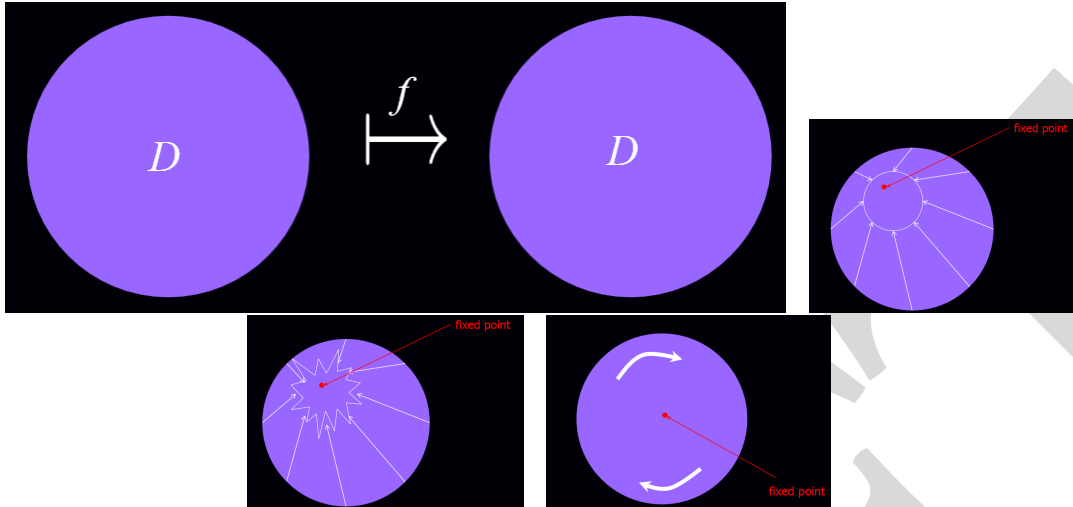
Figure 22.4: Brouwer's Fixed Point Theorem
