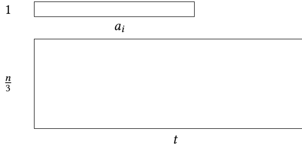
Figure 6.6: 3-PARTITION \leq restricted RECT-RECT PACKING
