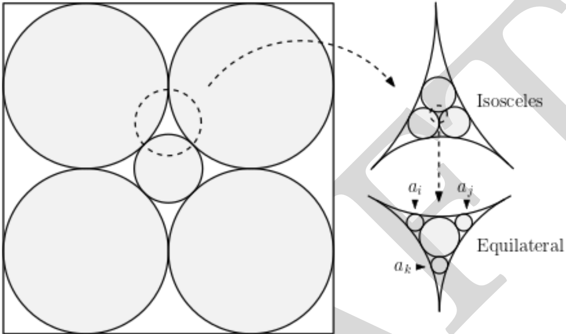
Figure 6.19: How to Adapt Disk Packing to a Square Instead of a Triangle.
