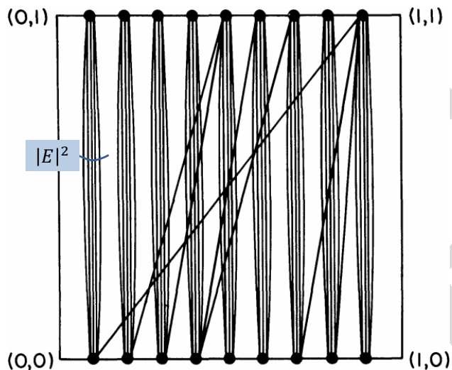
Figure 5.12: Bipartite Graph From Reduction of MINIMUM LINEAR ARRANGEMENT
