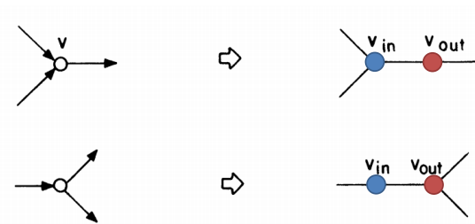
Figure 4.2: Reduction from PLANAR DIRECTED DEGREE-3 HAM to PLANAR UNDIRECTED BIPARTITE DEGREE-3 HAM.
