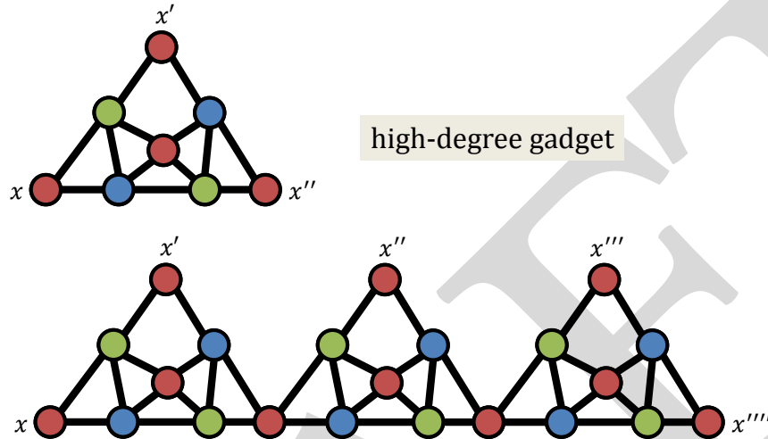
Figure 2.13: Gadget for Reducing Degree to 4
