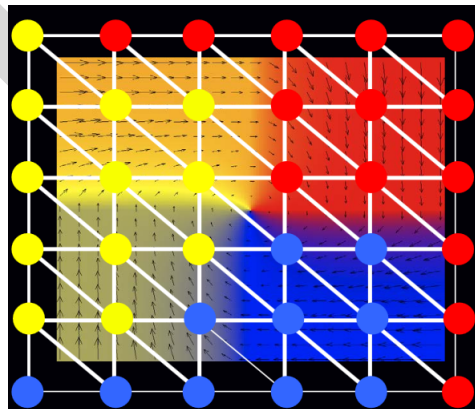
Figure 22.9: The Overlay of Sperner's Coloring on a Function Mapping [0, 1]^2 \rightarrow [0, 1]^2
