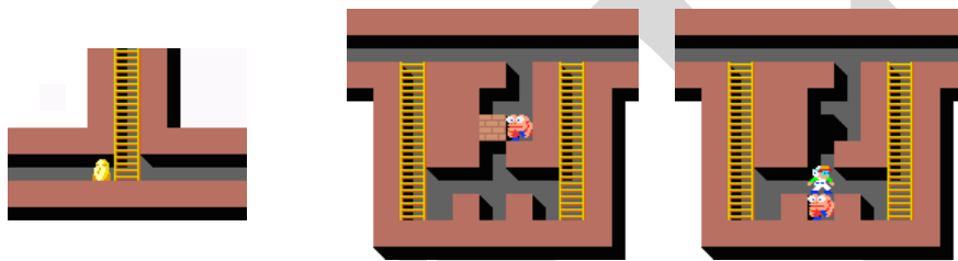
Figure 4.13: (Left) Location traversal gadget. (Center) Single-use path gadget and (right) it being used.
