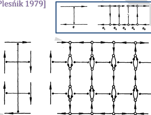
Figure 4.1: Gadgets for Proving HAM CYCLE on Planar Max-Degree-3 Graphs is NP-Complete
