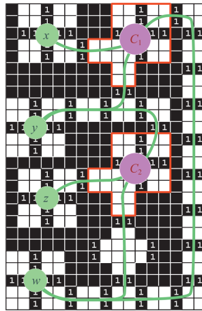
Figure 2.18: Shakashaka Puzzle Encoding a Planar 3SAT Instance Using Variable, Clause and Wire Gadgets
