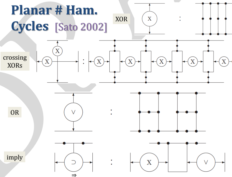
Figure 12.4: Gadgets for XOR, Crossing XOR, OR, Imply
