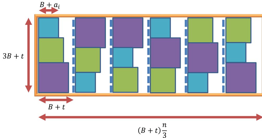
Figure 6.7: 3-PARTITION \leq SQ-RECT PACKING
