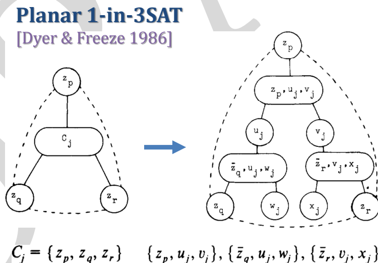
Figure 12.1: PLANAR 1-IN-3SAT Reduction Transformation
