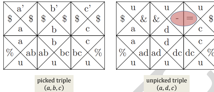
Figure 10.2: Gadgets for EM \leq_L 3D\text{-MATCHING-2}
