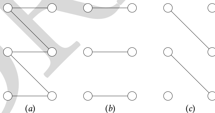
Figure 12.10: (a) Bipartite Graph (b) Perfect Matching (c) Maximal Matching
