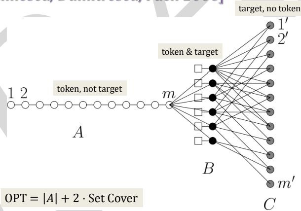
Figure 10.4: SET COVER \leq_L MOTION PLANNING Modified
