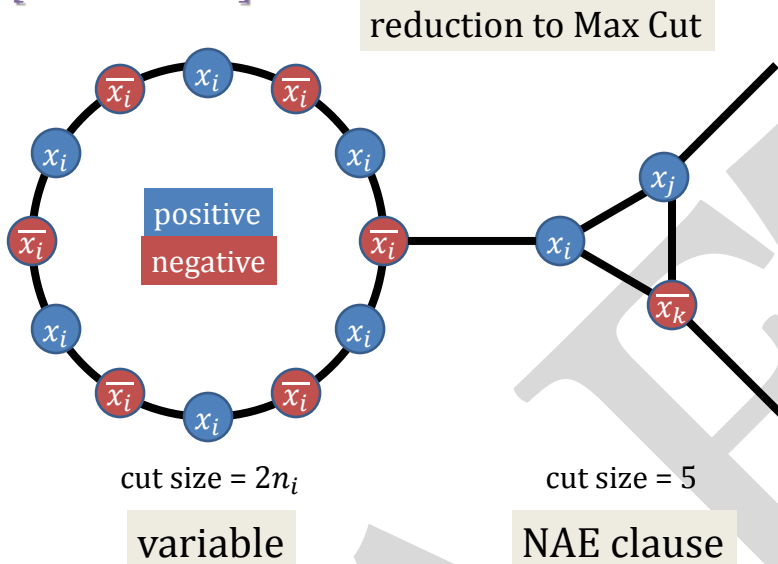
Figure 2.23: Gadgets for Planar NAE 3SAT to Planar Max Cut
