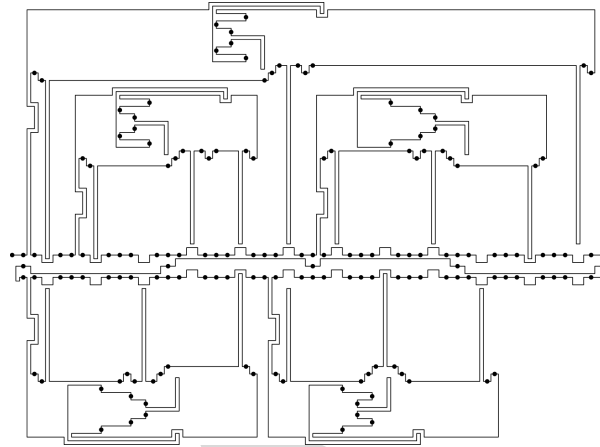
Figure 2.24: Fixed-angle Chain-Flattening Instance Encoding a Planar Monotone Rectilinear 3SAT Instance.
