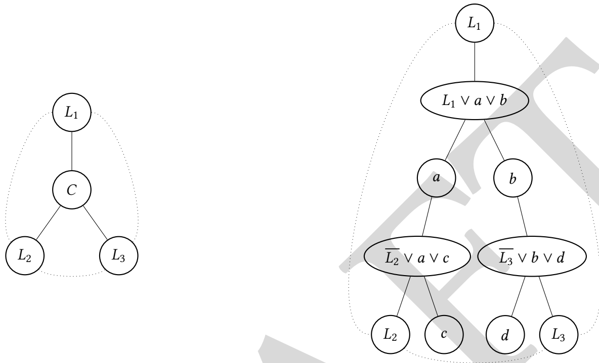
Figure 2.21: \text{PLANAR 3SAT} \leq \text{PLANAR 1-IN-3SAT}
