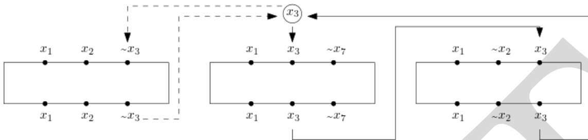
Figure 12.9: Gadgets For Variables in Proof PERM is #P-hard
