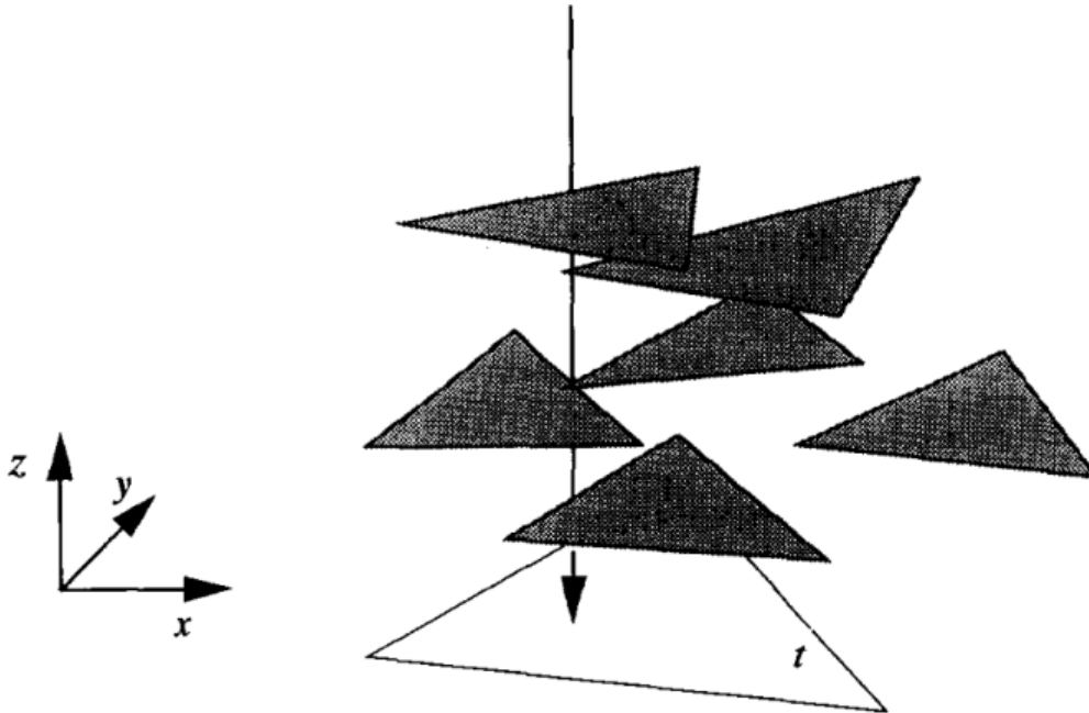
Figure 17.8: Visible Triangle Reduction
