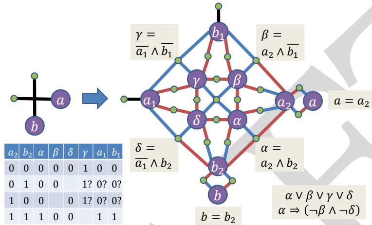
Figure 2.3: Planar 3SAT Crossover Gadget
