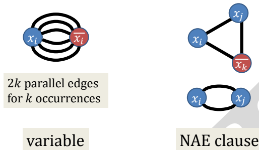
Figure 10.1: MAX NAE-3SAT \leq_L MAX CUT
