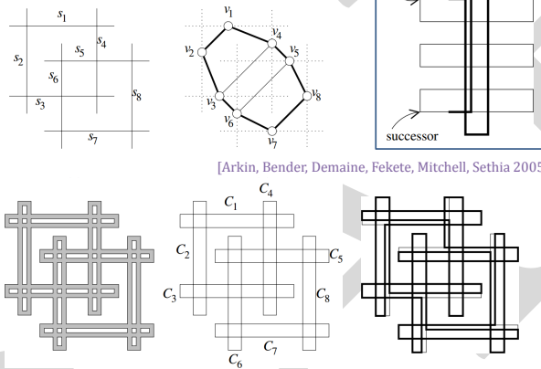
Figure 4.11: Gadget For Showing Hashiwokakero is NP-Complete
